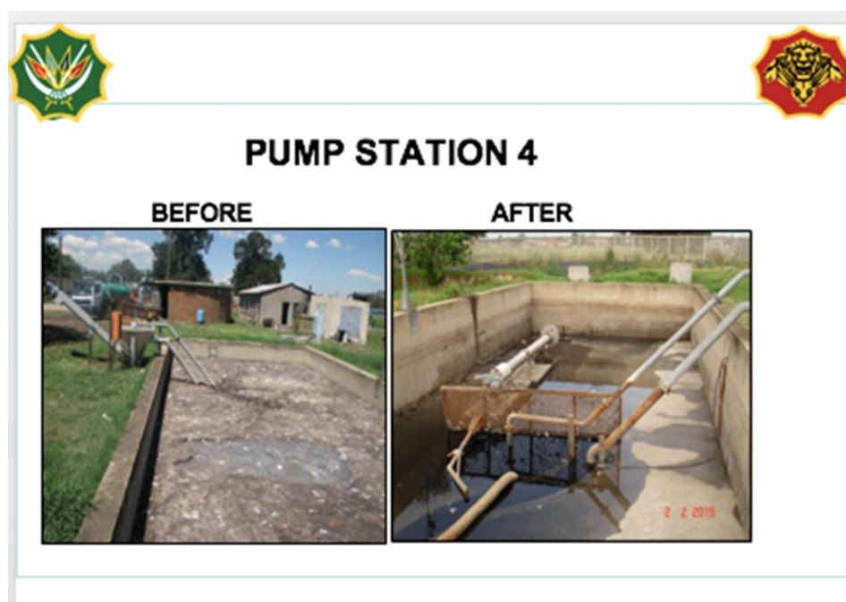
Diagram 1: Pump Station 4
